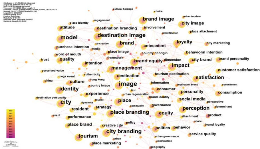
Figure 1: Co-occurrence network of keywords
