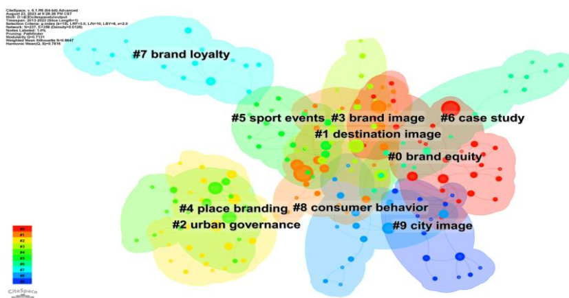
Figure 2: Cluster Graph of Keywords
