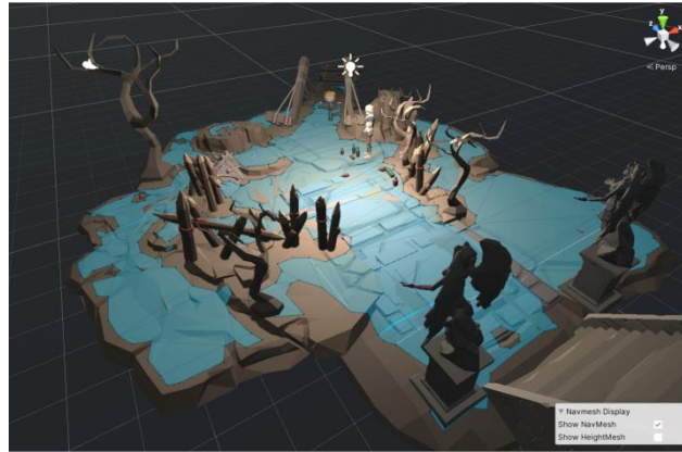
Figure 4: NavMesh area.
