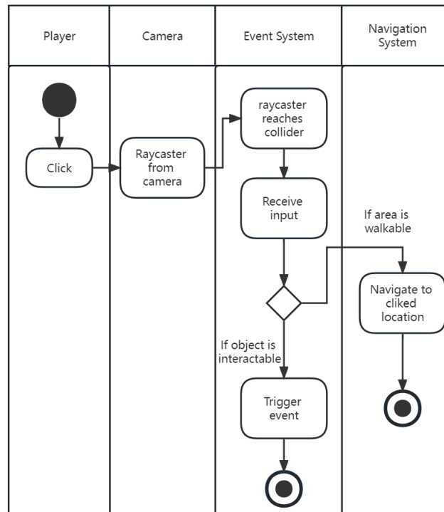
Figure 5: Player controller activity diagram.
