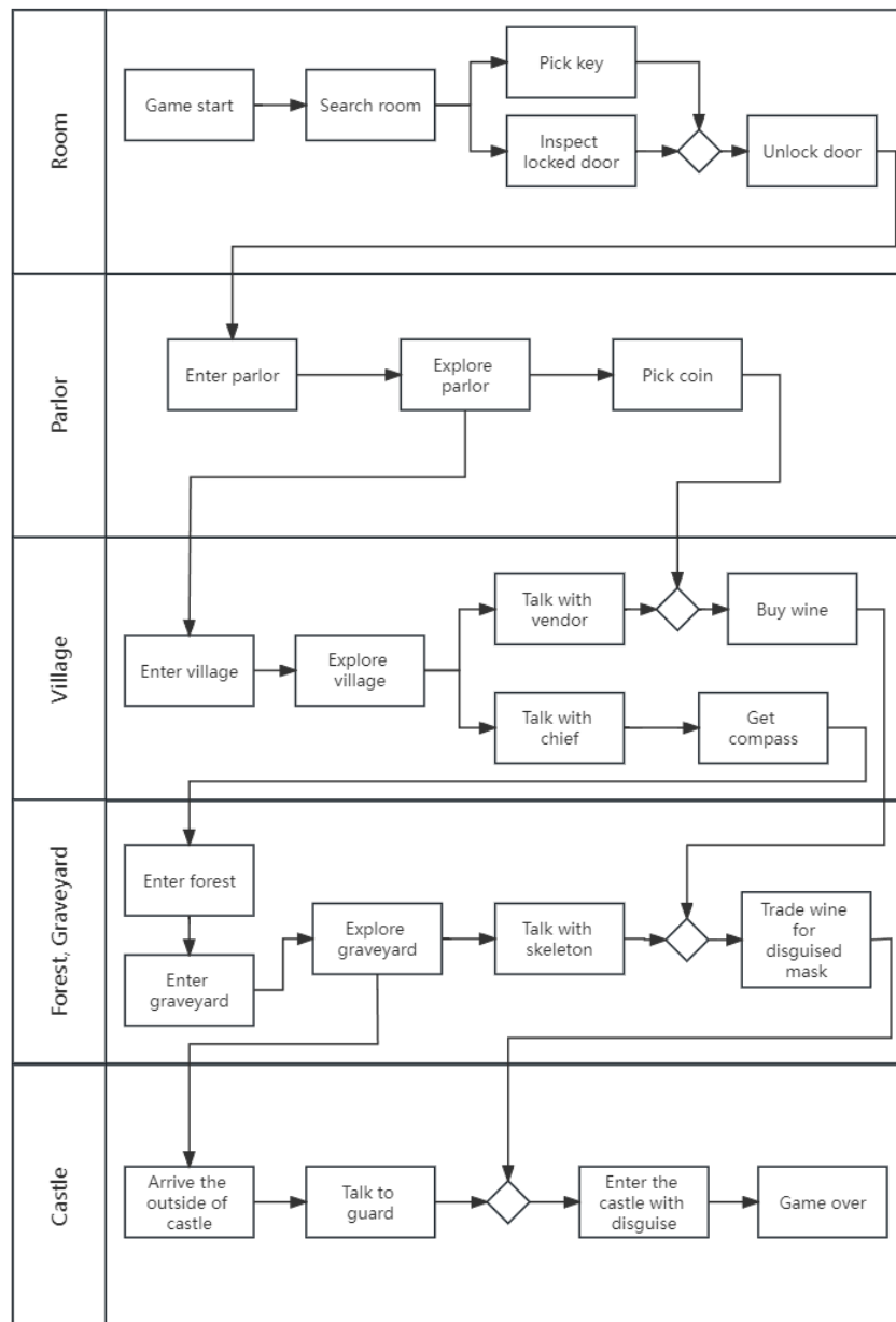
Figure 3: Puzzle-solving diagram.
