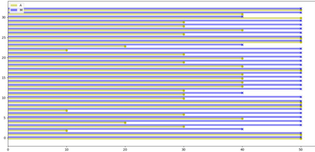
Figure 1: Test results of Experiment 1 “Ancient Chinese and Modern Standard Chinese” (Horizontal: test score; Vertical: participant number).
