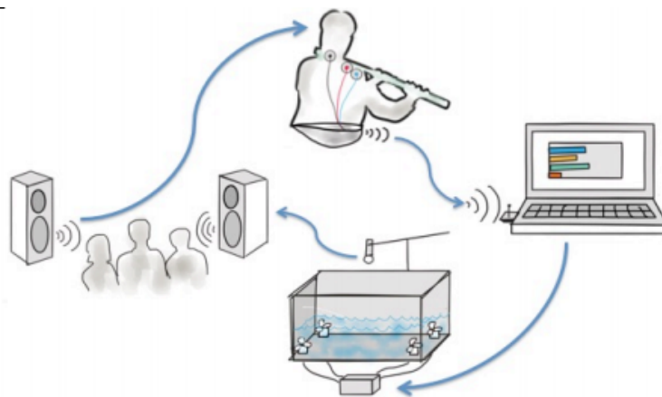
Figure 2. The torrent system, showing data flow. Source: [2]
