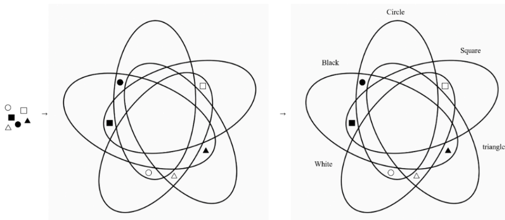
Figure 2. Object-driven construction
