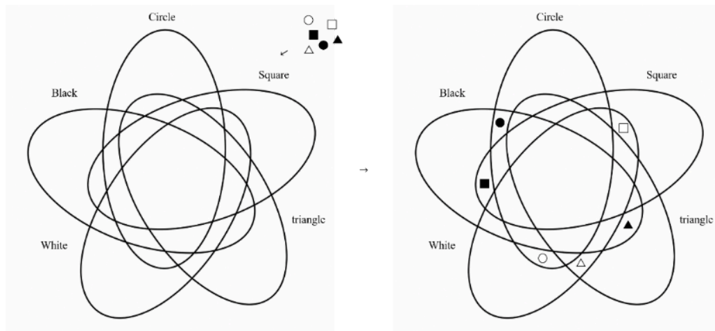
Figure 3. Predicate-driven construction
