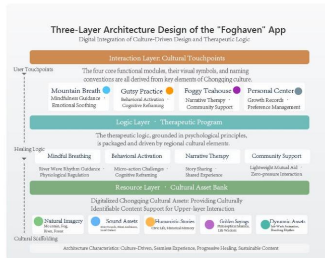
Figure 1. The Three-Layer architecture design of Foghaven
