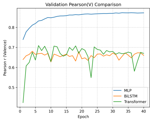
Figure 1. Validation Pearson correlation curves for Valence (picture credit: original)
