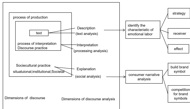
Figure 1. Analysis flowchart
