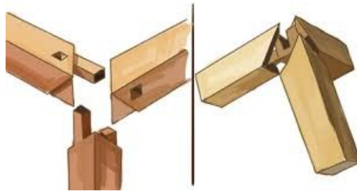
Figure 6. Tenon-and-mortise joint [15]
