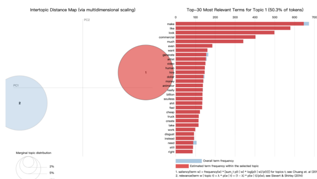
Figure 7. Top 30 most relevant terms for topic 1
