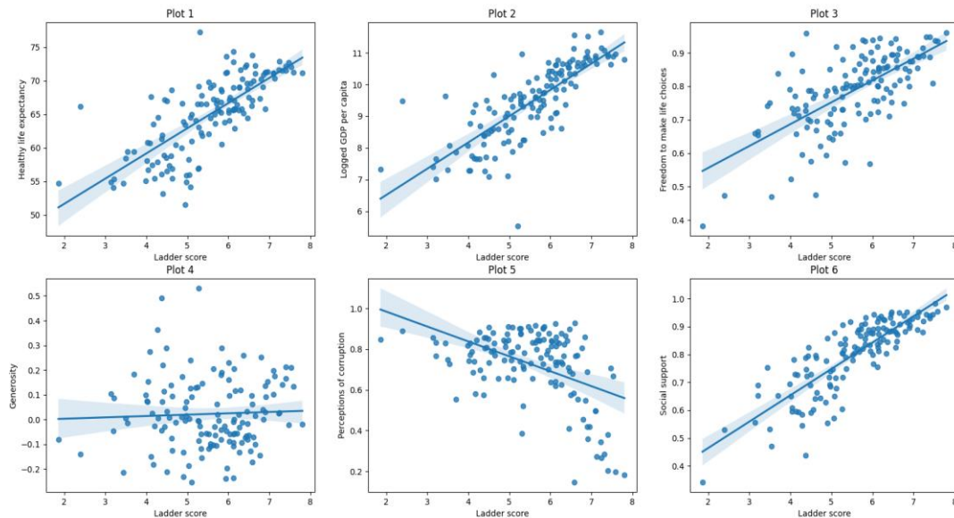
Figure 3: scatter plots
