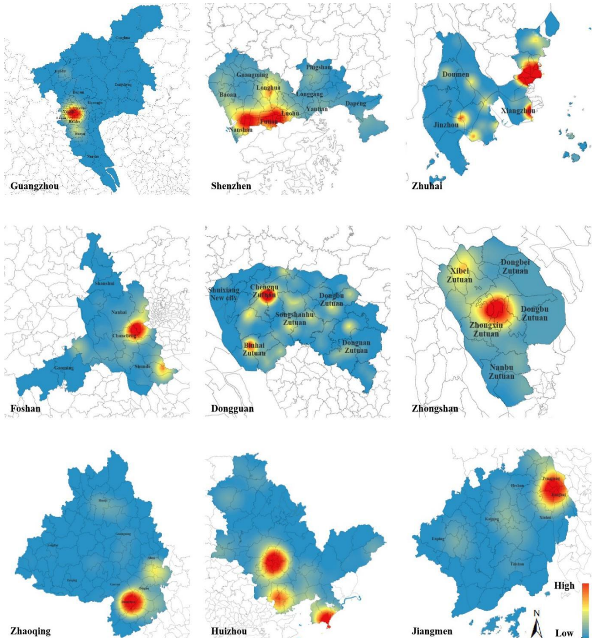
Figure 5: The result of Kernel density estimation in each city of the PRD.
